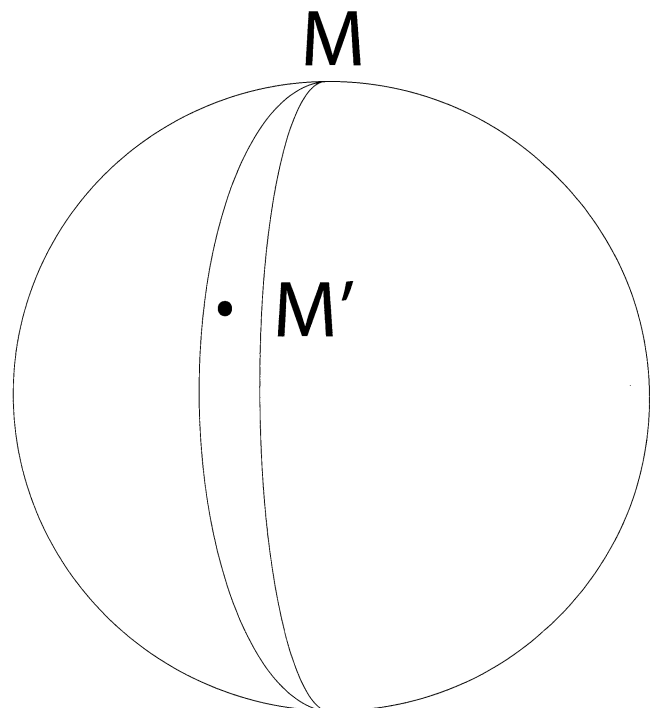
FIG. 1. Borel's Figure 13.
