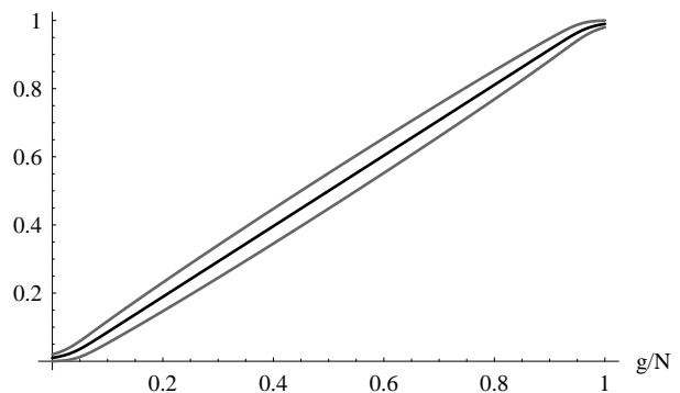
FIG. 7: Plot of \mu(P|G = (g, N - g)) and \sigma(P|G = (g, N - g)) (depicted as the grey curves \mu \pm \sigma ) as a function of g/N for N = 100 and values of \alpha = 0.1 and \beta = 0.2 .
